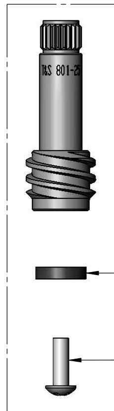
000801-25 Removable Spindle, LTC Qty = 1 ea.
