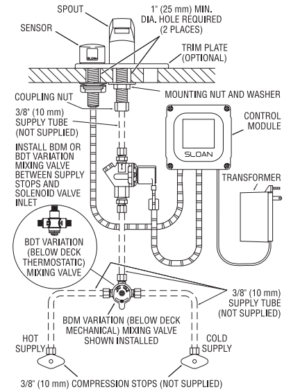
ETF-660 Faucet with BDM and BDT Variation Mixing Valves for Hot and Cold Water Supply (shown with 4" trim plate)
