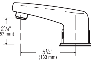
ETF-660 Lavatory Faucet
