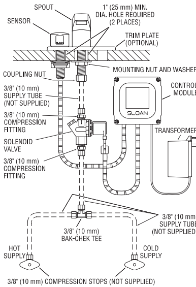
ETF-660 Faucet with Bak-Chek® Tee for Hot and Cold Water Supply (shown with 4" trim plate)
