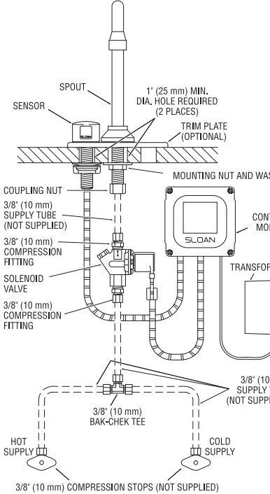
ETF-770 Faucet with Bak-Chek® Tee for Hot and Cold Water Supply (shown with 4" trim plate)
