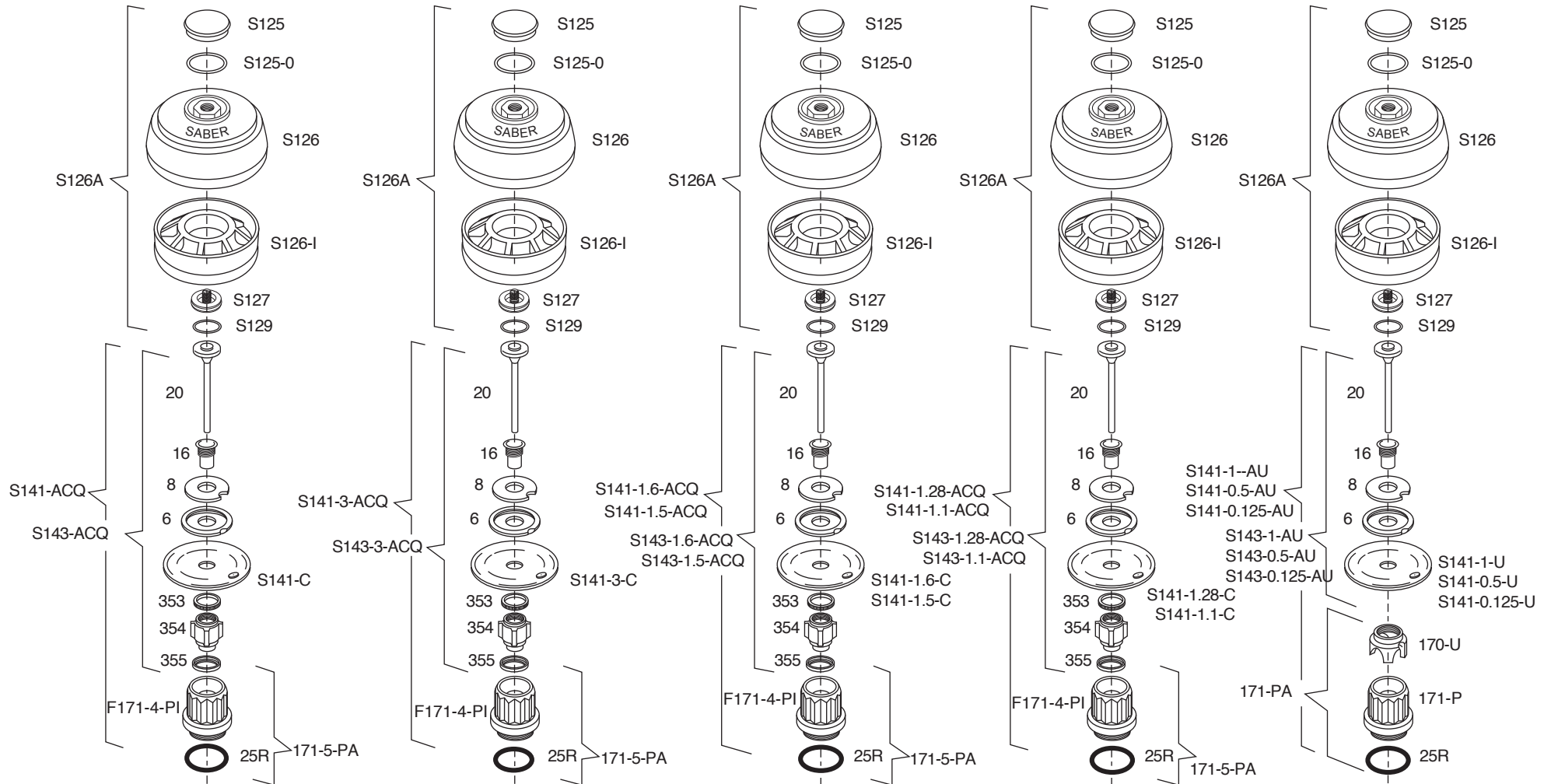
S402 / S452 (Valves with 1" supply)
