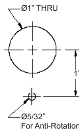
EC-3100 & EC-3102 MOUNTING HOLE DIAGRAM
